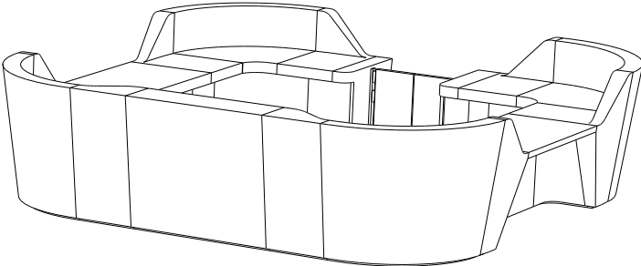
Example 1 Made up of modules; HQ- S2D1 LH, HQ- IM4 1000, HQ- S2D2 RH, HQ- LM4 RH, HQ- L2H4 DDA RH, HQ- LM2 1000, HQ- L2H3 DDA RH, HQ- LM4 RH, HQ- L2H2 RH, HQ- EM2, HQ- GATE, HQ- EM1, HQ- L2H1 LH, HQ- CM3 LH, HQ- L2H4 DDA RH, HQ- LM2 1000, HQ- L2H3 DDA LH, HQ- CM3 LH
