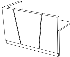
Module Name: Left Hand High Module 1750 Module Code: Z-EMH1 /1750 Module Size: 1750x750x1100mm
