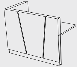
Module Name: Left Hand High Module 1450 Module Code: Z-EMH1 /1450 Module Size: 1450x750x1100mm
