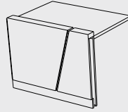
Module Name: Middle Low Module 1000 Module Code: Z-MML / 1000 Module Size: 1000x750x800
