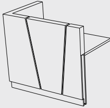
Module Name: Left Hand High Module 1250 Module Code: Z-EMH1 /1250 Module Size: 1205x750x1100mm
