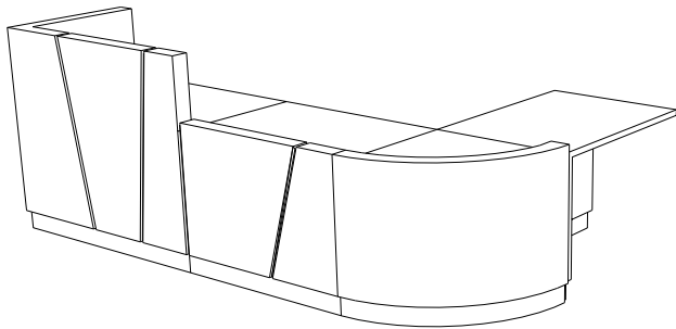
Example 1 Made up of modules; Z-EMH1 / 1250, Z-MML / 1000, Z-LRCE / 750, Z-DDA / 1000
